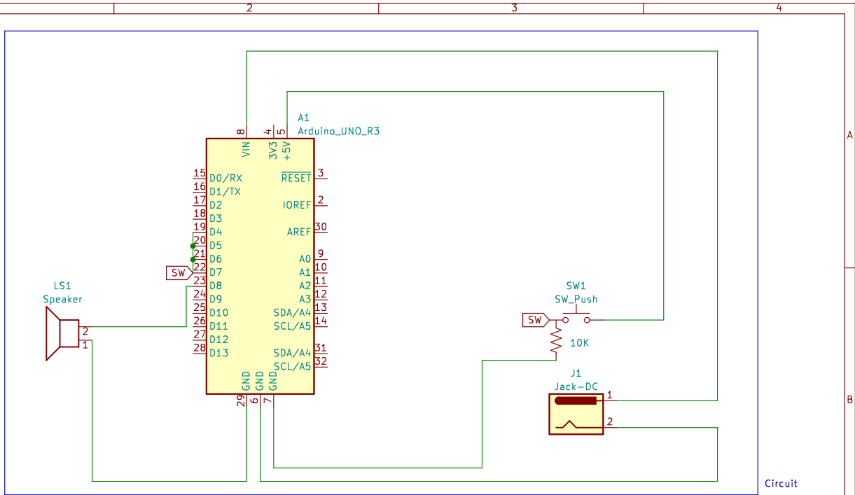
Circuit
